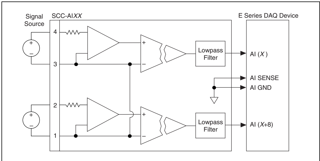
Figure 1-1. SCC-AIXX Signal Connections
