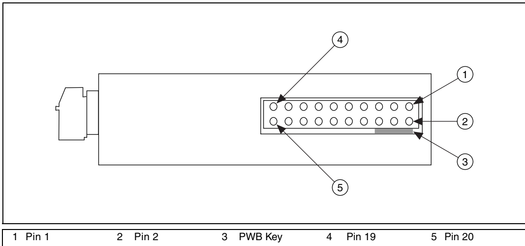
Figure 1-4. SCC Module Bottom View
