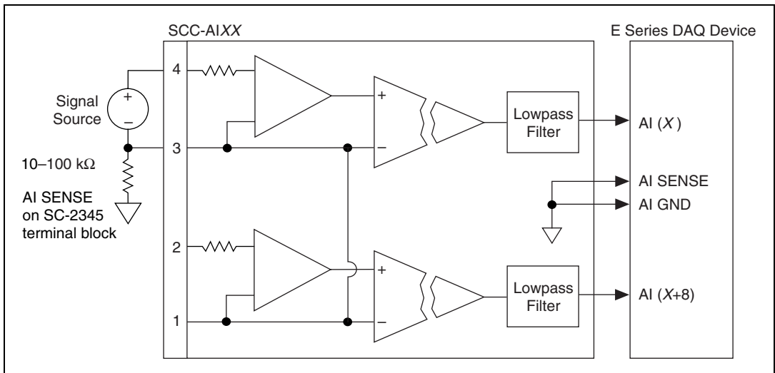
Figure 1-2. Nonreferenced Signal Connection for the SCC-AIXX (One Channel)
