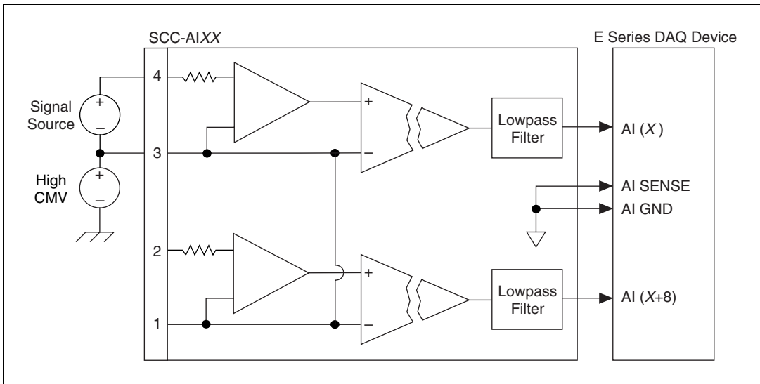
Figure 1-3. Ground-Referenced Signal Connection for the SCC-AIXX with High Common-Mode Voltage (One Channel)
